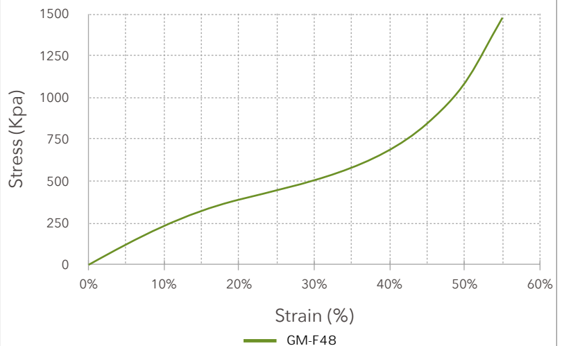
GM-F series CFD Curve
