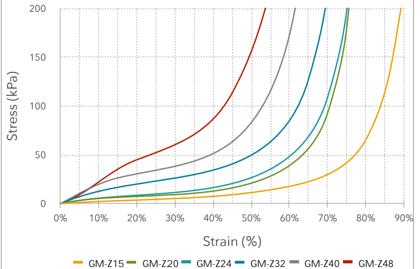
GM-Z series CFD Curve
